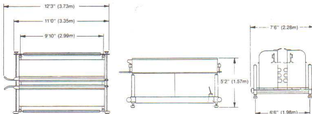
10' Standard Cabinet Drawings are for layout purposes only.
